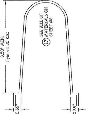
0.187" DIA. WIRE ANCHOR
