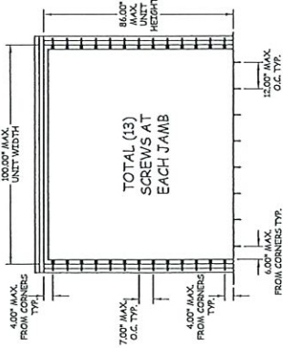
3/8" DIA. LAG SCREWS ANCHOR LOCATION INSTALLATION INTO WOOD STRUCTURE
